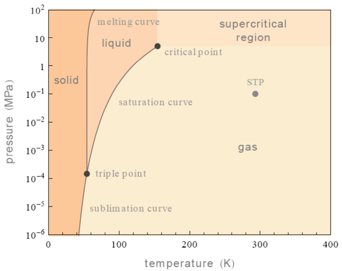
Phase diagram: oxygen
