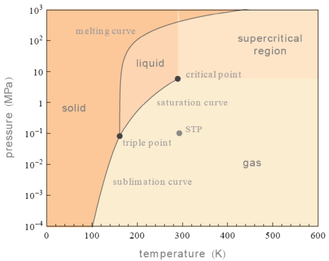
Phase diagram: xenon
