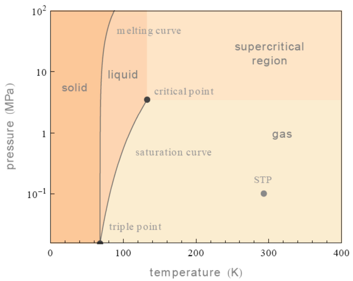
Phase diagram: carbon monoxide
