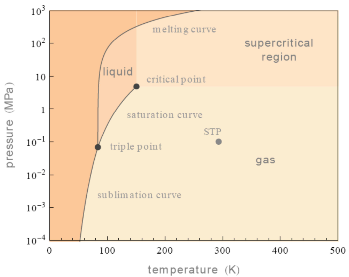
Phase diagram: argon
