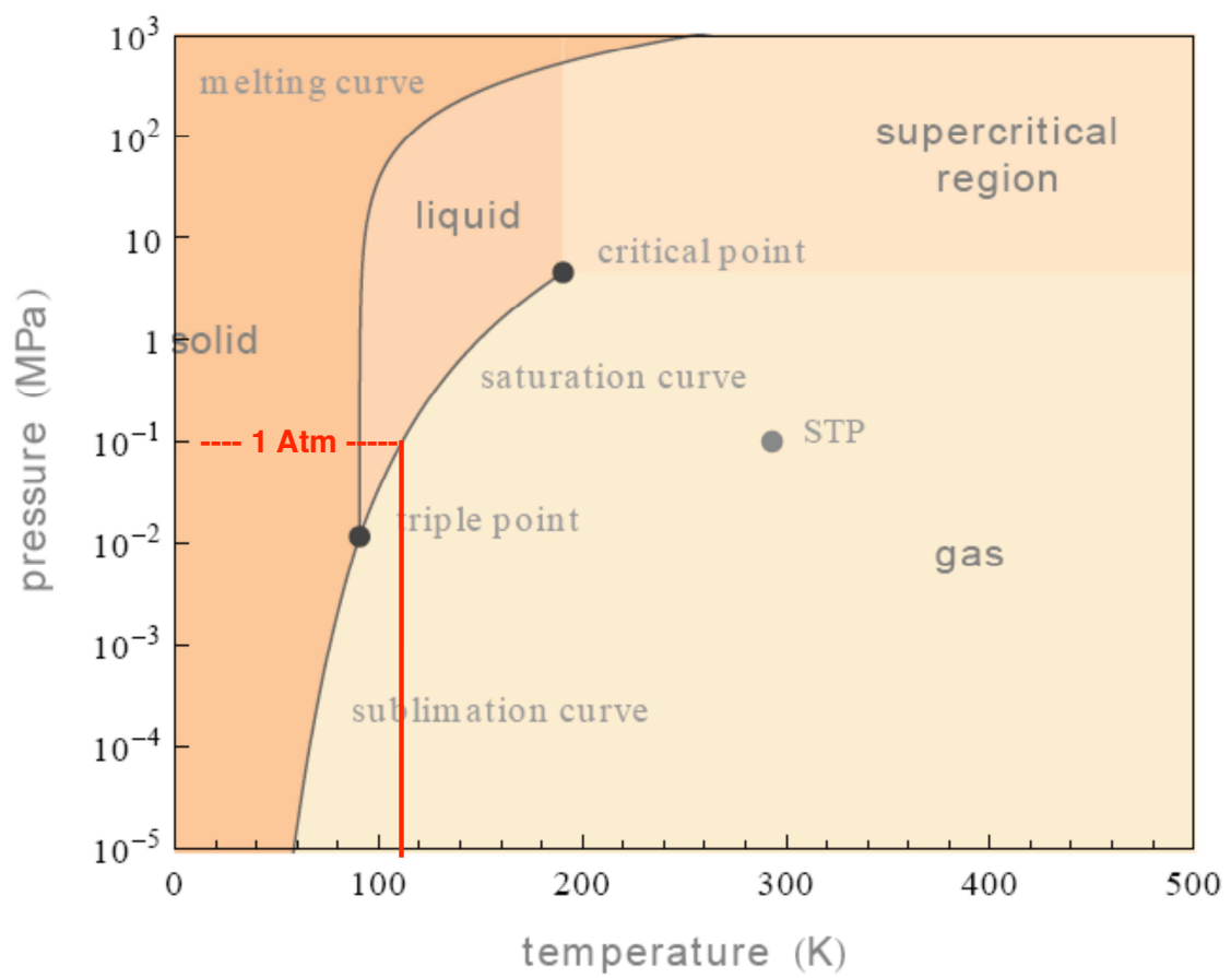
Phase diagram: methane
