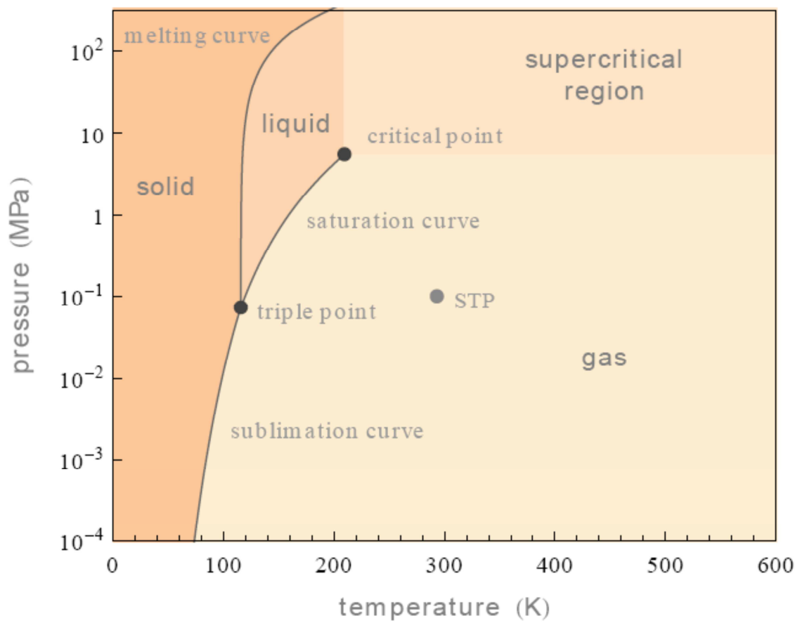
Phase diagram: krypton
