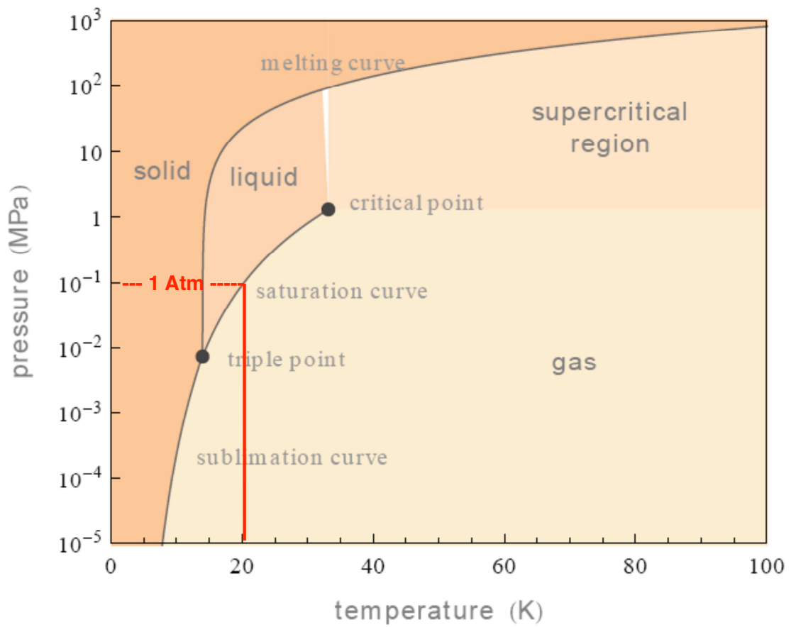
Phase diagram: hydrogen
